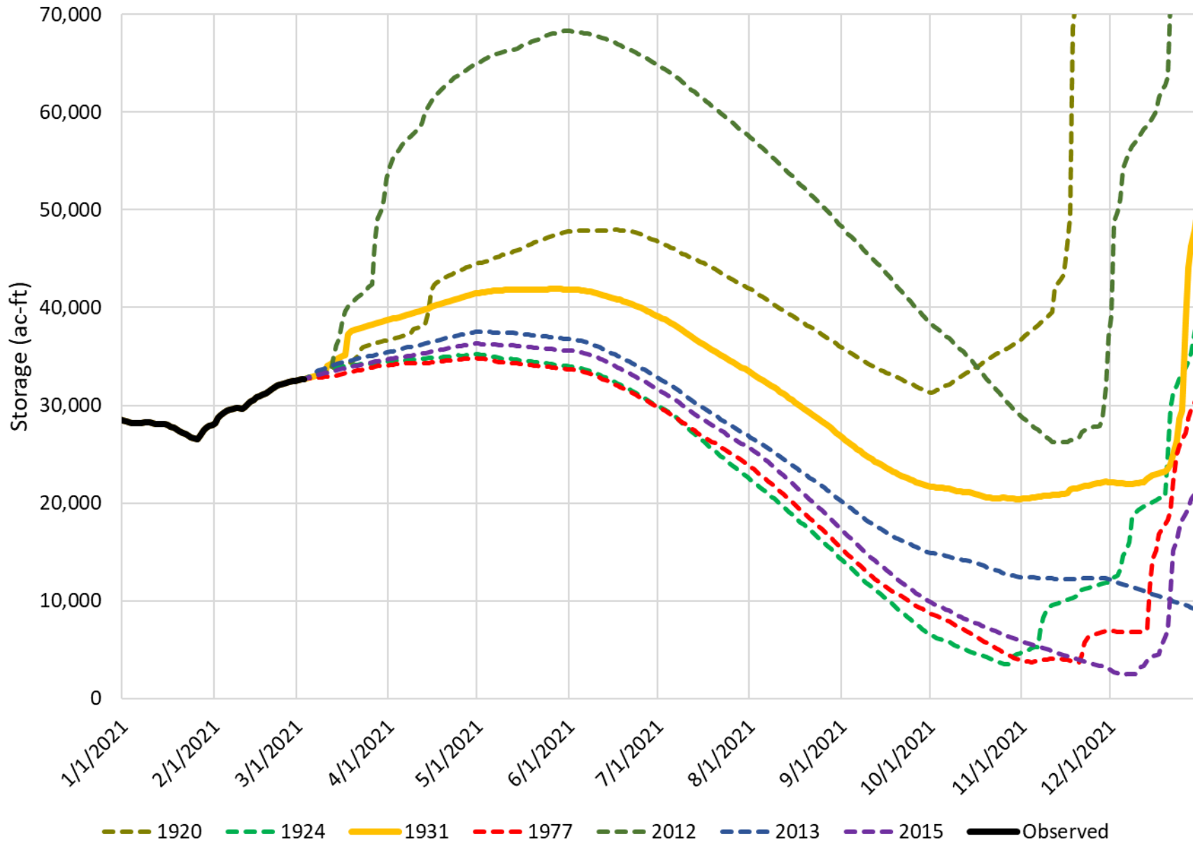
Lake Mendocino Storage (Projection Feb 26, 2021)
