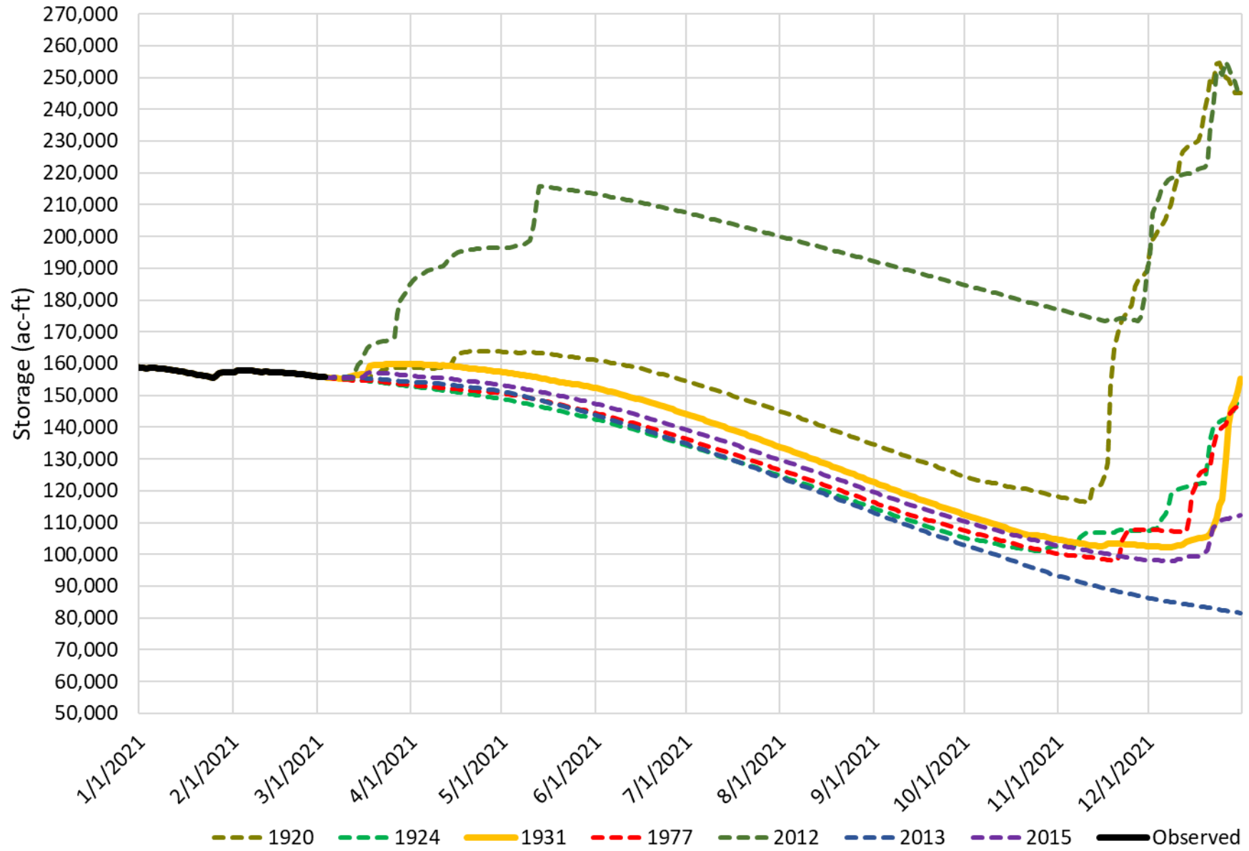
Lake Sonoma Storage (Projection Feb 26, 2021)
